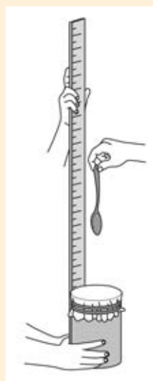
Opstelling.
