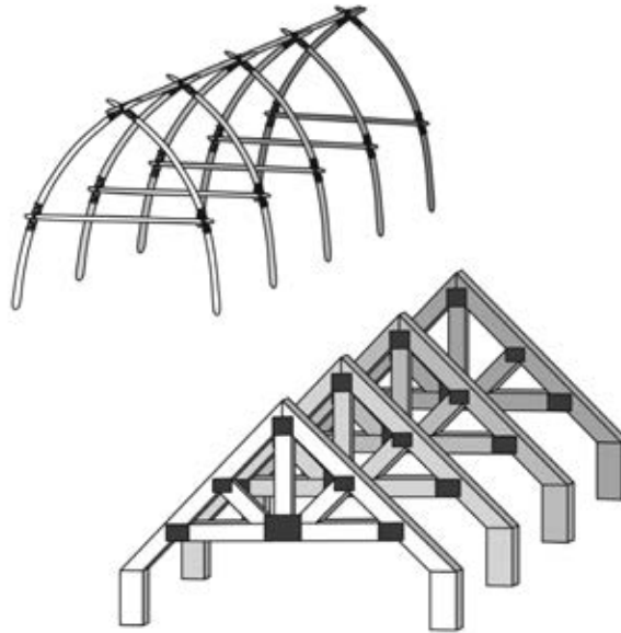
Traditional and modern structures
